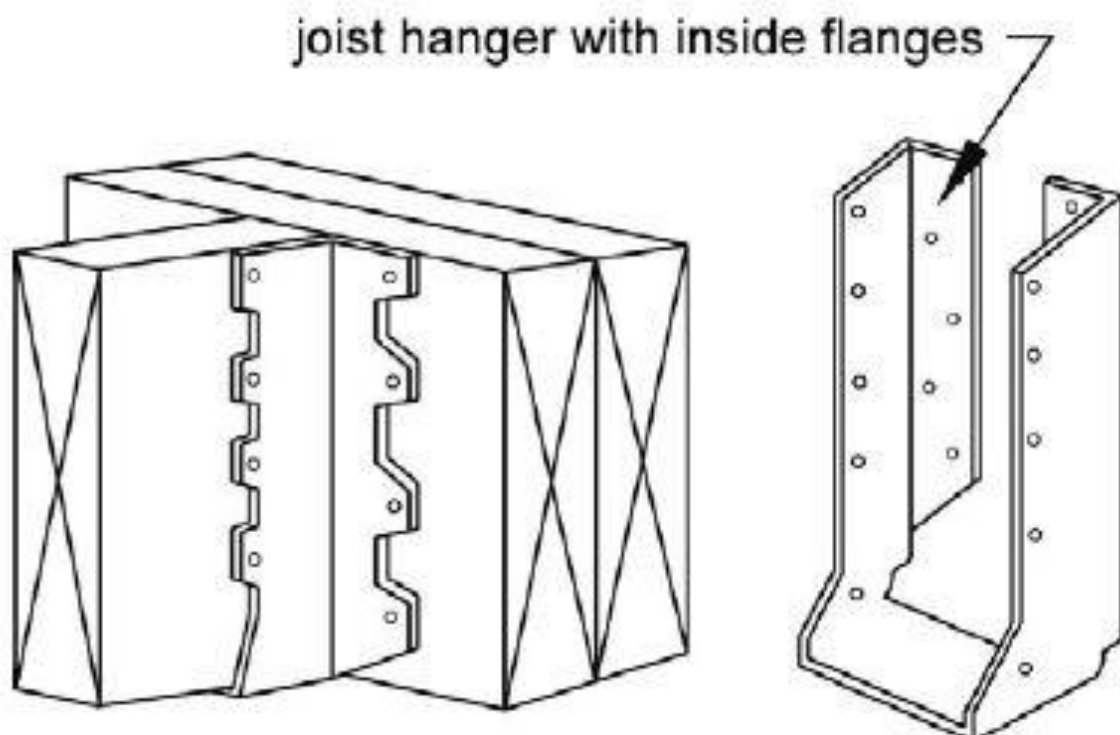
Figure 7. Typical Joist Hangers.
