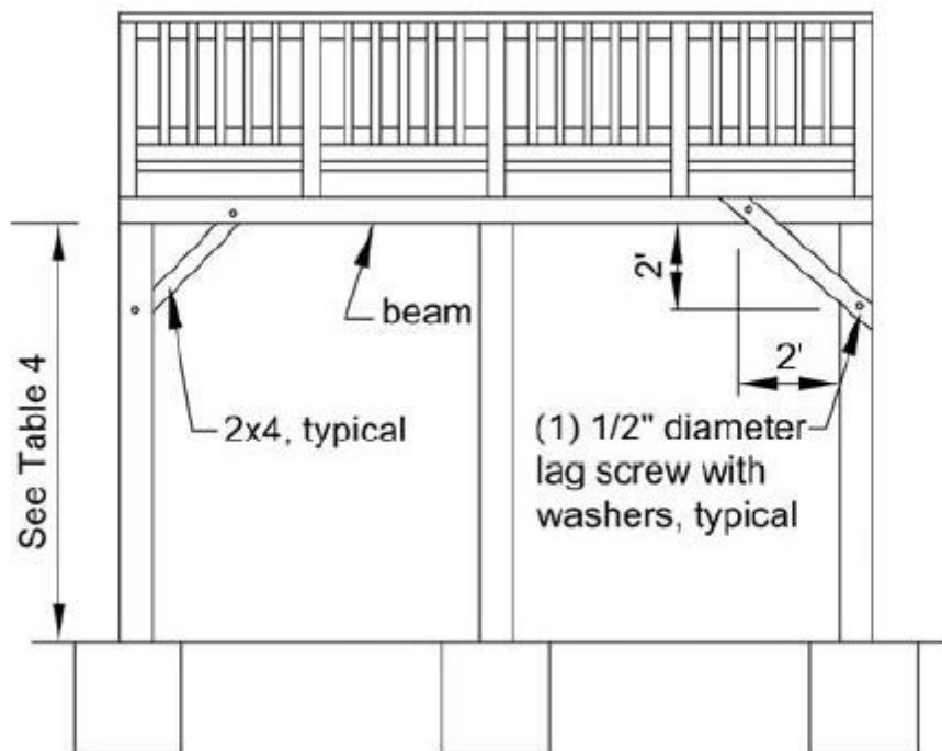
Figure 10. Diagonal Bracing.
