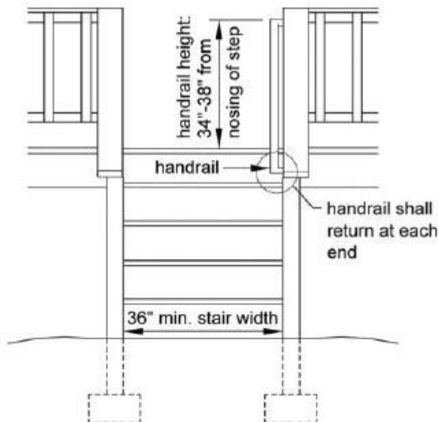
Figure 33. Miscellaneous Stair Requirements.
