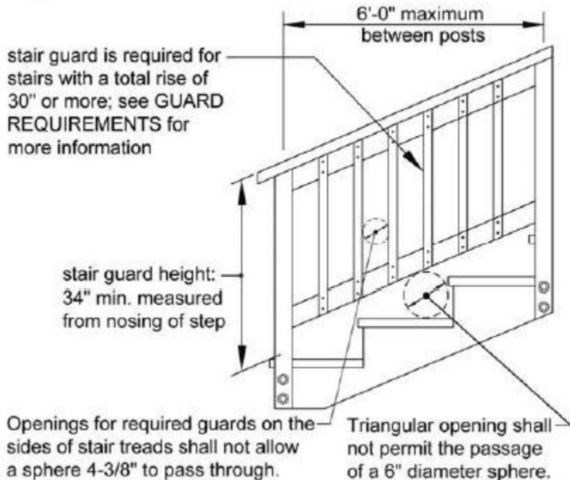
Figure 30. Stair Guard Requirements.
